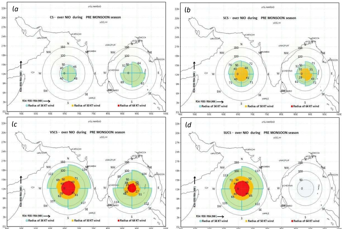
Fig .1.6 (a).Quadrant wind radii of 34 (green), 50 (yellow) and 64 (red) knots wind (R34, R50 and R64) in association with TCs of different intensities (a) CS, (b) SCS, (c) VSCS and (d) SuCS during pre- monsoon season. The values written inside each quadrant indicate mean R34, R50 and R64 (nautical miles)
