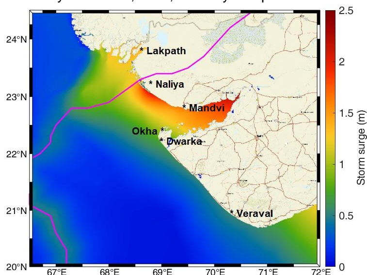
Fig. 5.16: Estimated Storm surge in association with ESCS Biparjoy during landfall
