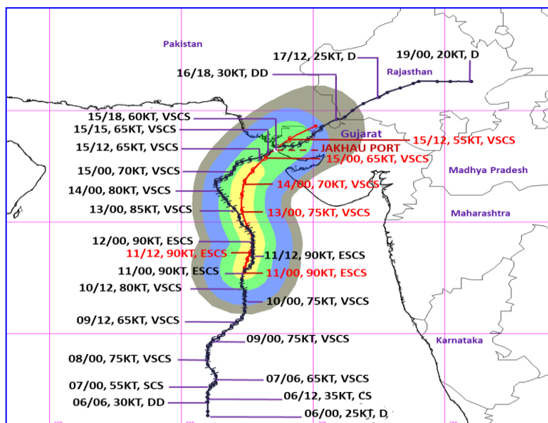
Fig.6.12. Typical example of radii of quadrant wind forecast on 11th June based on 0000 UTC for ESCS Biparjoy
