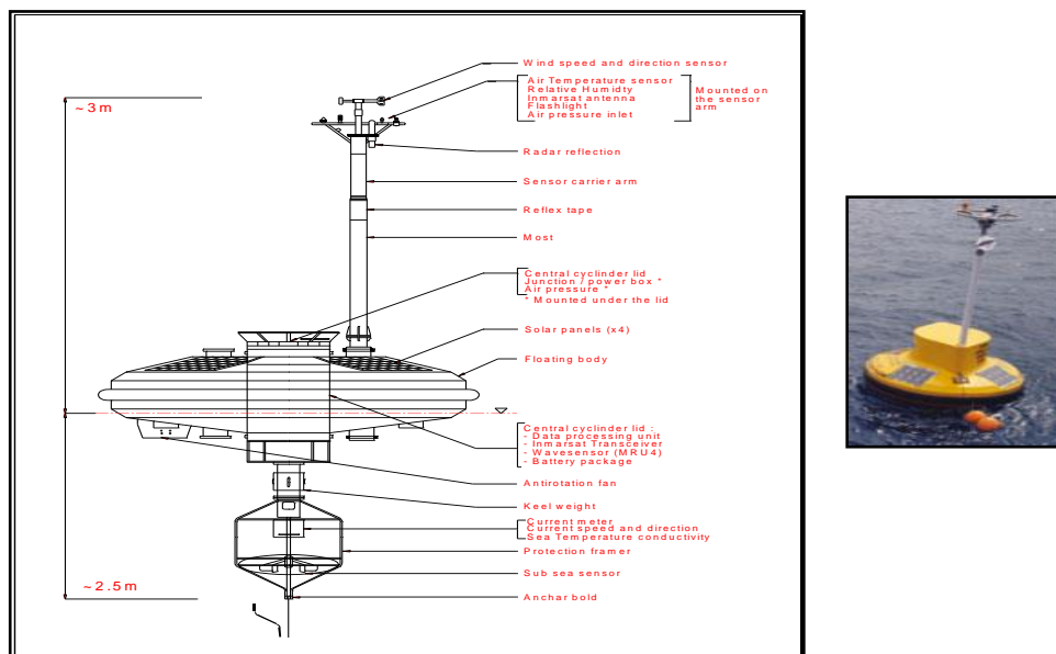
Fig.4.2. Picture of a Data Buoy deployed at Sea
