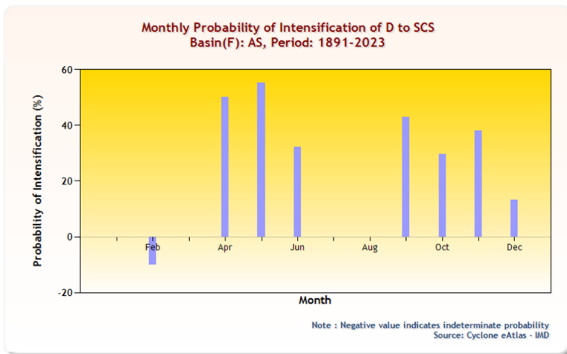
Fig.1.23 (f). Monthly Probability of intensification of depression into a severe cyclonic storm over AS during 1965-2023
