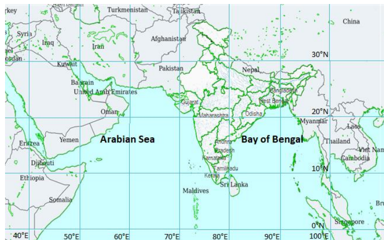
Fig 2.3 Area of responsibility of RSMC- Tropical Cyclones, New Delhi
