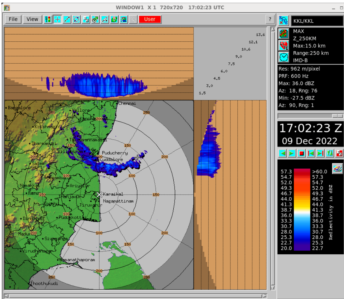
Image from Doppler Weather Radar Karaikal at 17 UTC.
