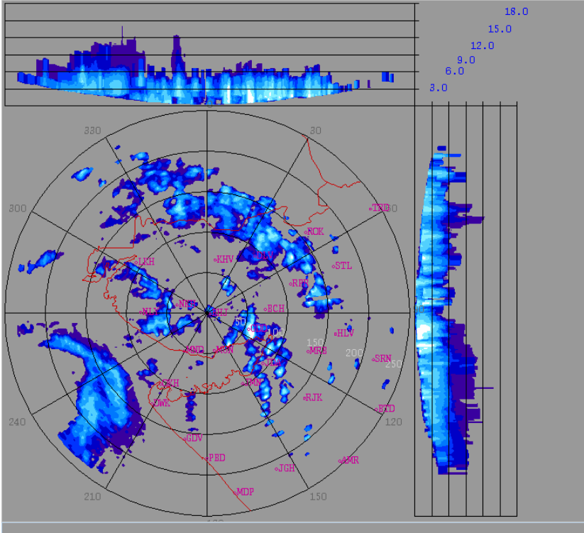
Reflectivity imagery from Doppler weather Radar -Bhuj based on 1250 hrs IST of 15 th June 2023.
