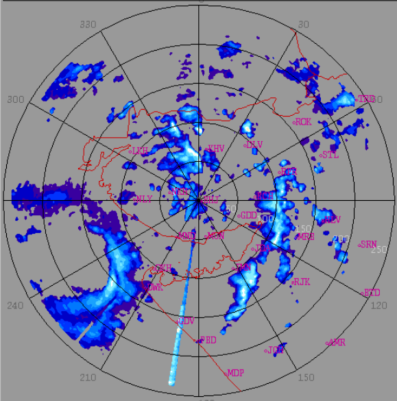
Reflectivity imagery from Doppler weather Radar -Bhuj based on 1620 hrs IST of 15 th June 2023.
