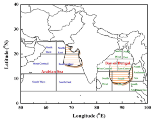
DAY-4: 02.12.2021/0600 UTC TO 03.12.2021/0600 UTC
