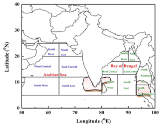
DAY-4: 02.12.2021/0600 UTC TO 03.12.2021/0600 UTC
