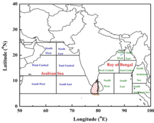
DAY-3: 01.12.2021/0600 UTC TO 02.12.2021/0600 UTC
