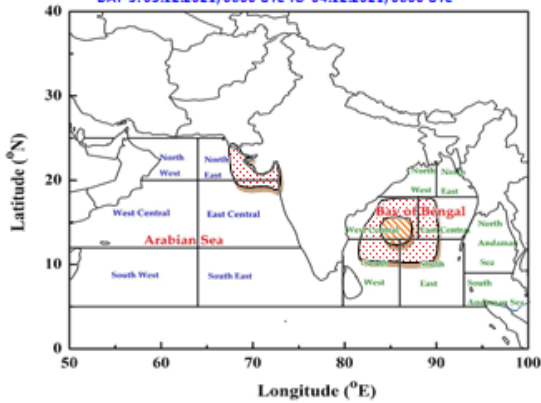
DAY-5: 03.12.2021/0600 UTC TO 04.12.2021/0600 UTC
