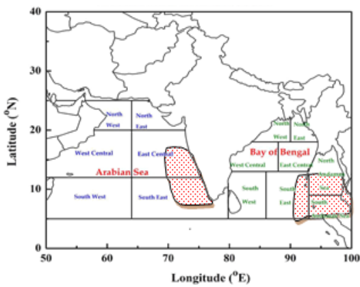
DAY-5: 03.12.2021/0600 UTC TO 04.12.2021/0600 UTC
