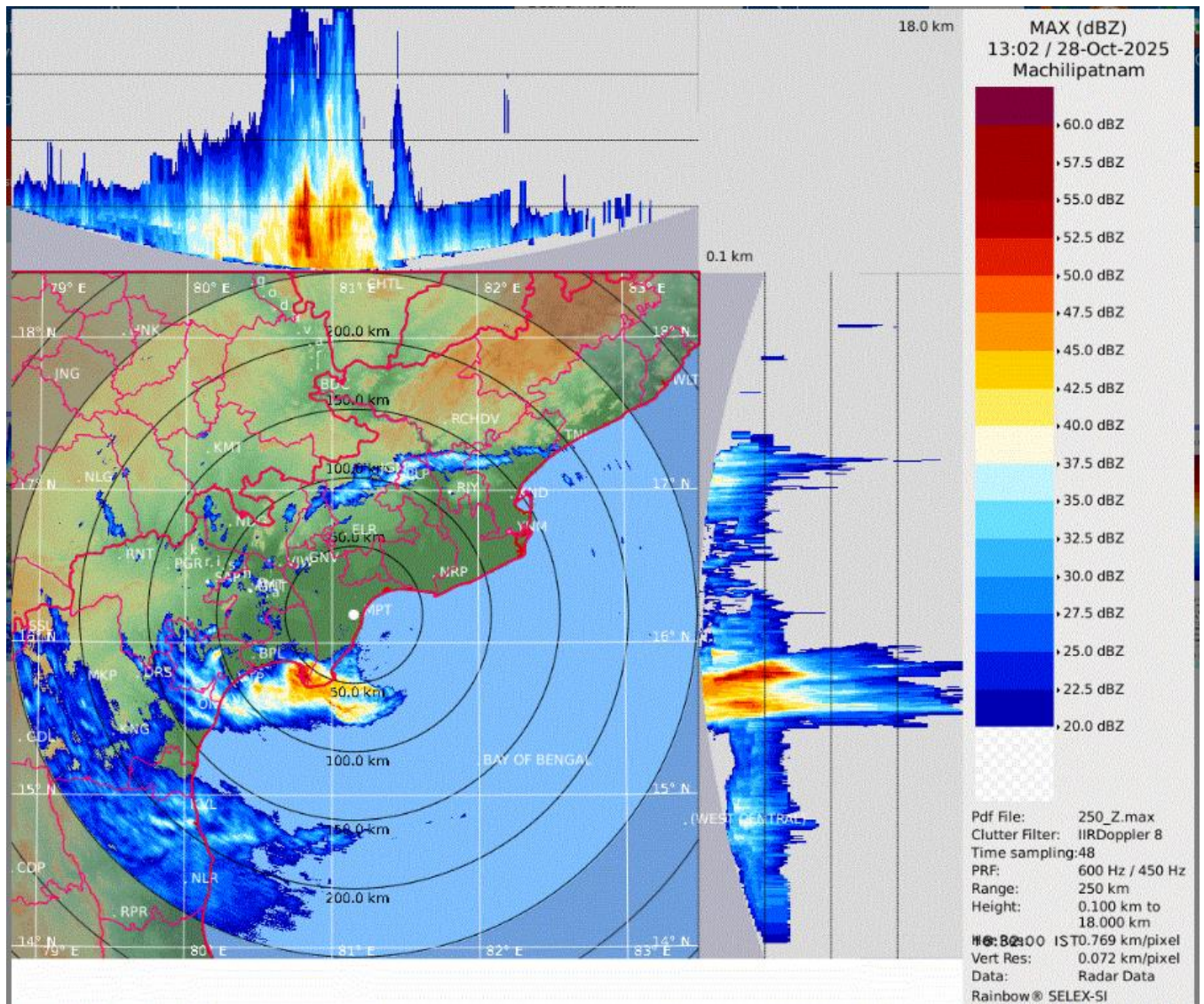
Max Z image of DWR Machilipatnam based on 1302 UTC (1832 IST) of 28 th October 2025
